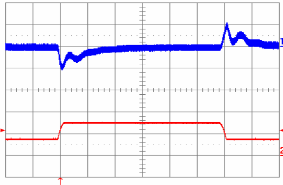
Fig. 20: Output voltage response to load current step-change (3.75 A – 7.5 A – 3.75 A) at V_{in} = 24\text{ V} . Top trace: output voltage (100 mV/div). Bottom trace: load current (5 A/div.). Current slew rate: 0.1 A/ \mu\text{s} . C_o = 1\ \mu\text{F} ceramic. Time scale: 0.2 ms/div.
